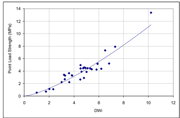
Figure 8 – Correlation Between Point Load Strength and the DW_i for a Copper Ore
