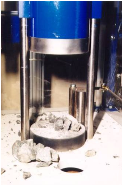
Figure 4 – Drop-weight Tester
