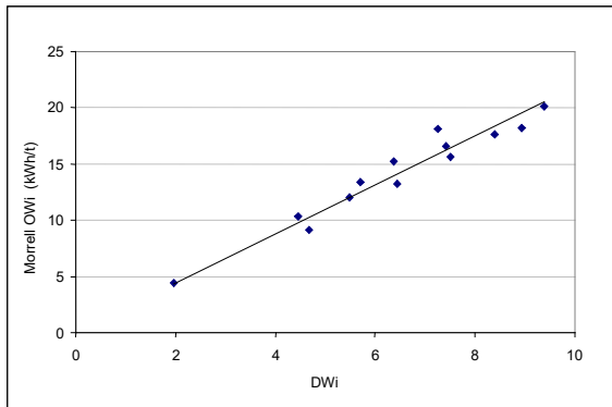
Figure 10 – DW i vs HPGR Operating Work Index
